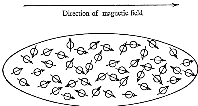
Fig. 1. Paramagnetism.
